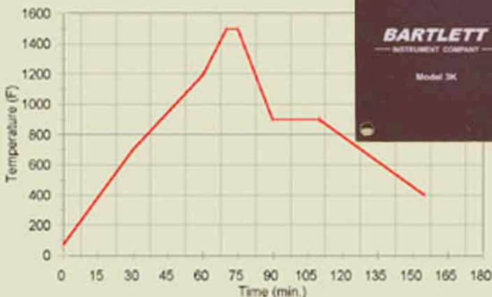
Sample Firing Profile Full Fuse, 90 COE Glass
